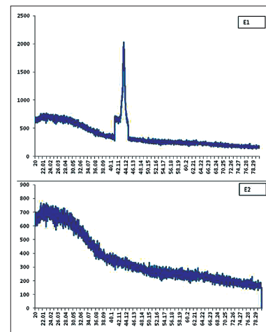
Figure 1: XRD pattern for E1 and E2
